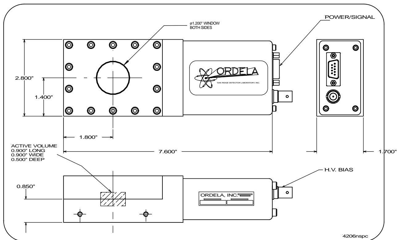
ORDELA Model 4206N Neutron Beam Monitor outline and dimensions
