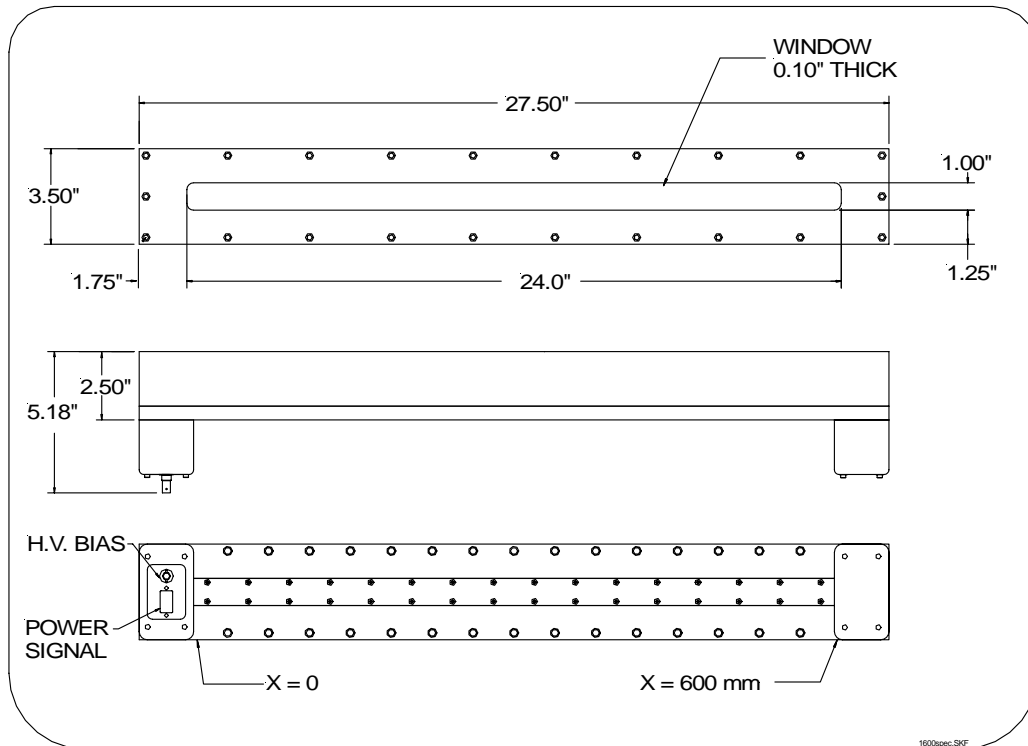
ORDELA MODEL 1600N OUTLINE AND DIMENSIONS
